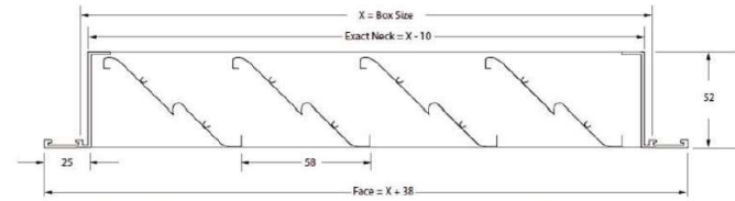
Dimensional Drawing:
