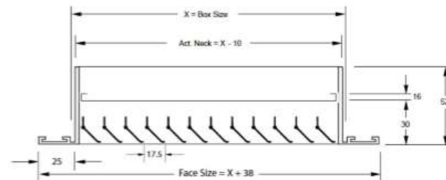
Dimensional Drawing:
